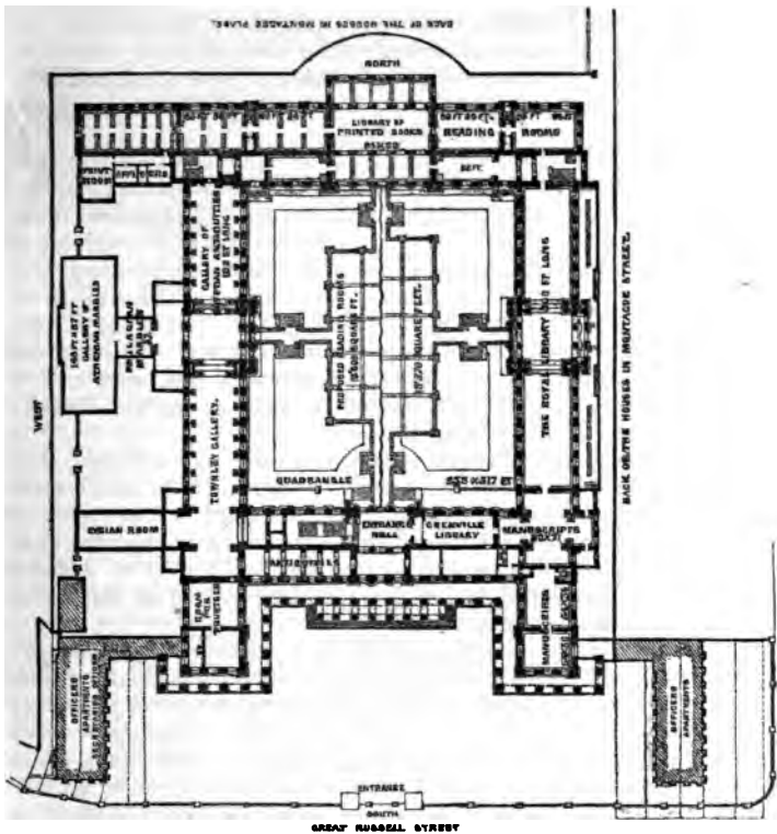
GROUND PLAN OF THE BRITISH MUSEUM.
